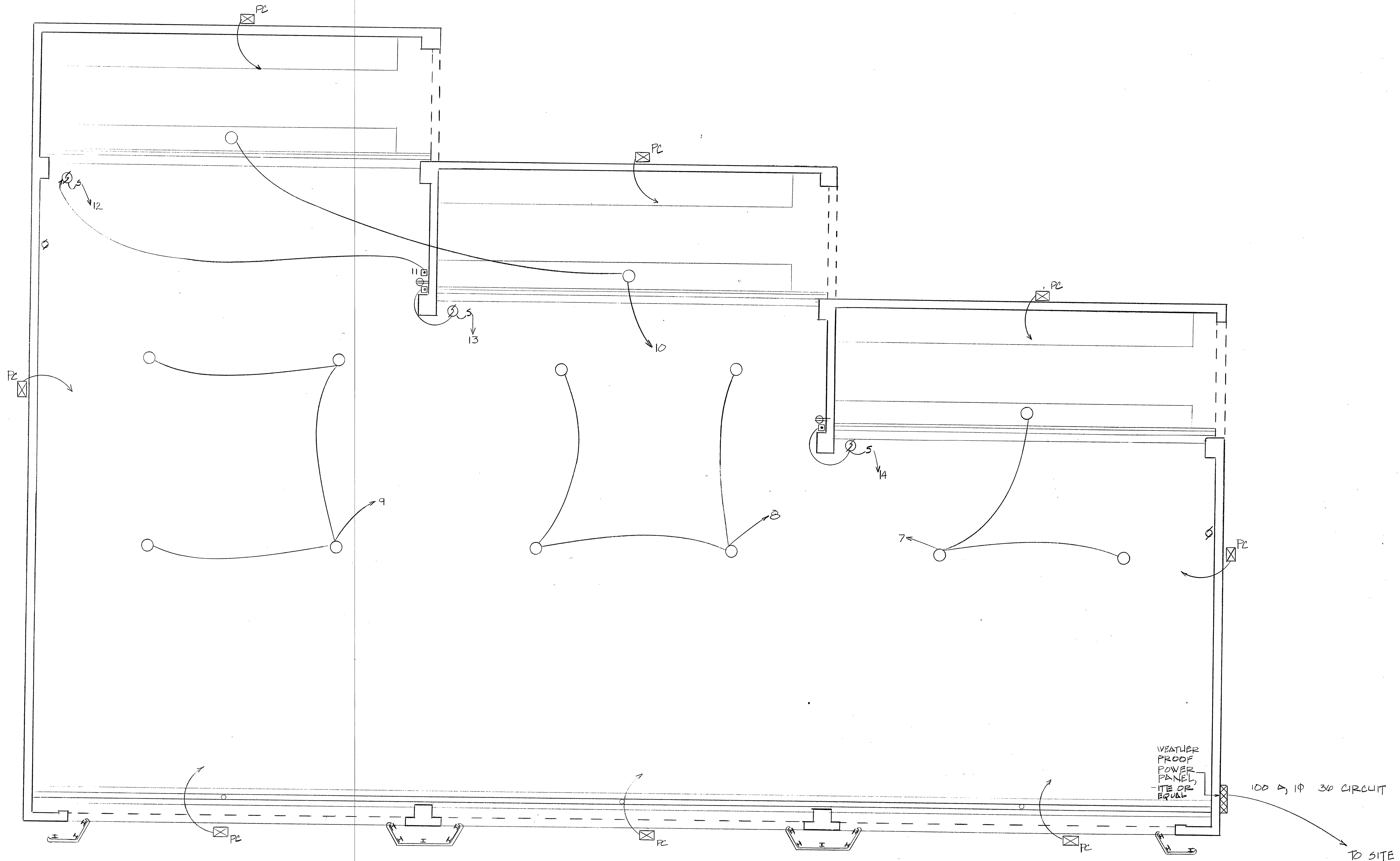
1 TIPPING FLOOR ELECTRICAL PLAN E2 SCALE: 3/16" = 1'-0"
