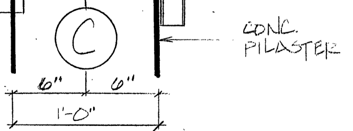
3 SECTION, DETAIL @ COL. LINE C SCALE: 1/2" = 1'-0"
