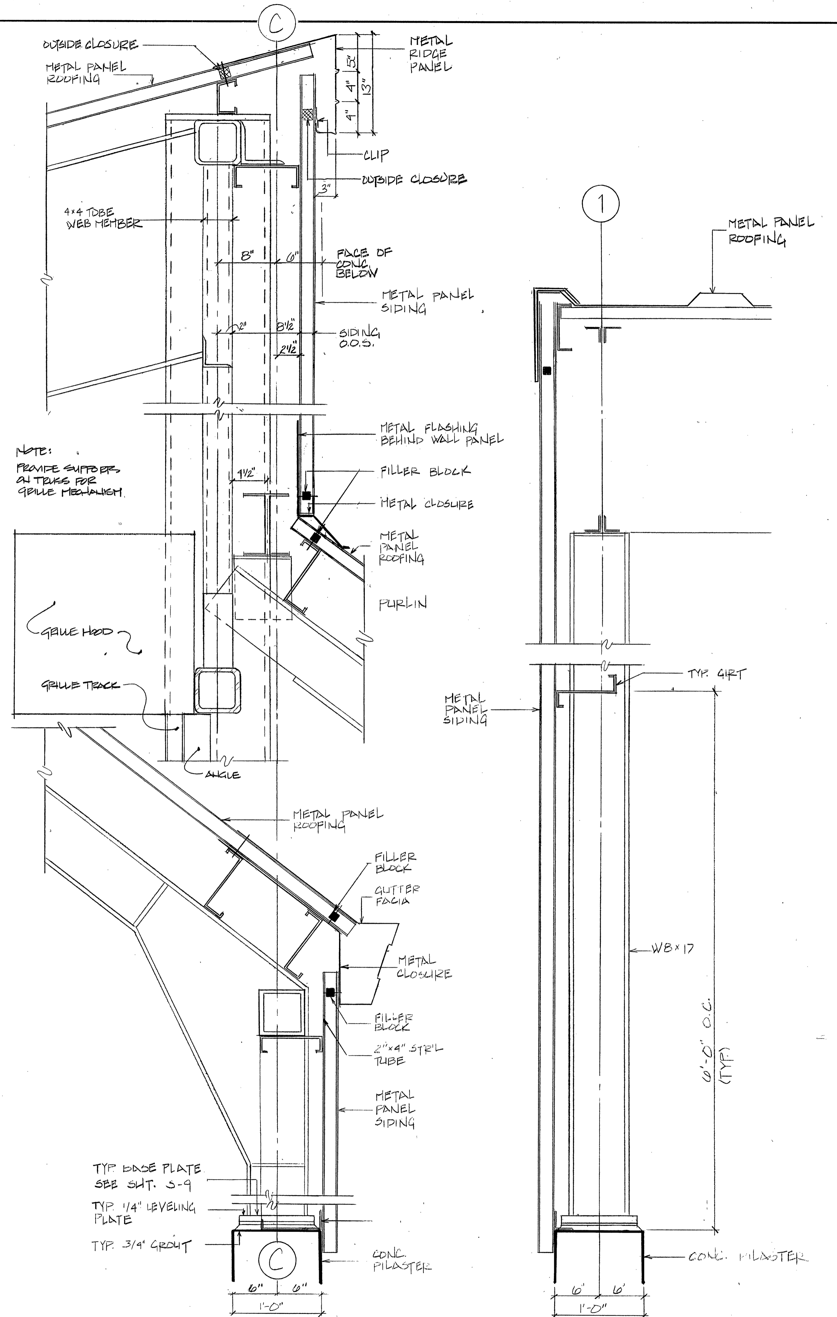
3 SECTION, DETAIL @ COL. LINE C SCALE: 1/2" = 1'-0"
