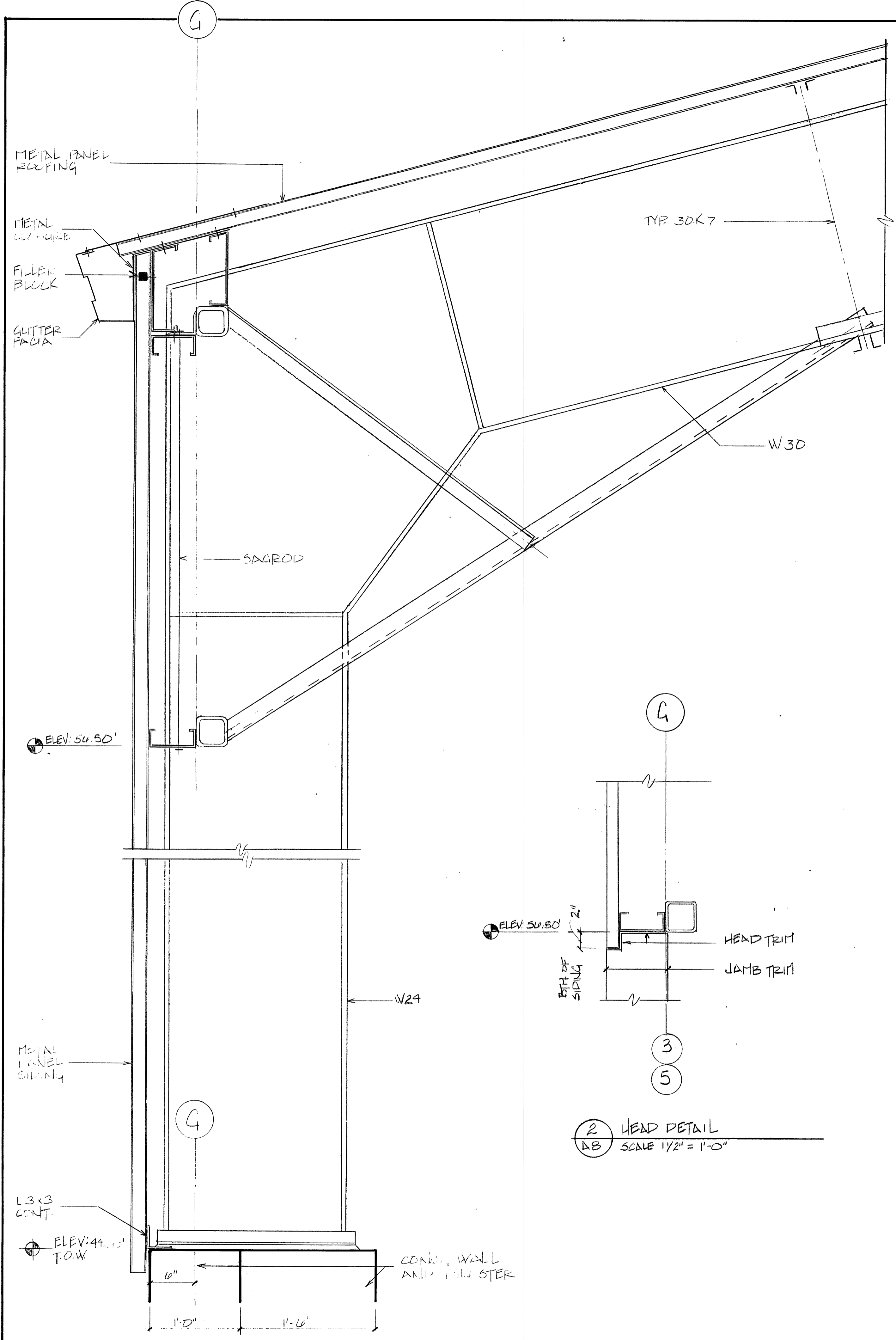
1 SECTION, DETAIL @ COL. G-3 & G-5 SCALE: 1/2" = 1'-0"
