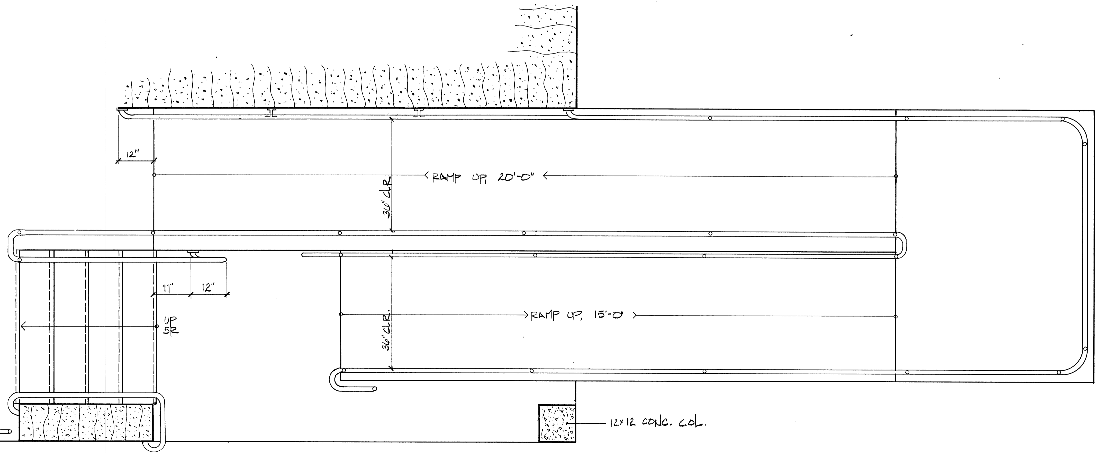
2 DETAIL-PLAN @ RAMP RAIL SCALE 3/4" = 1'-0"
