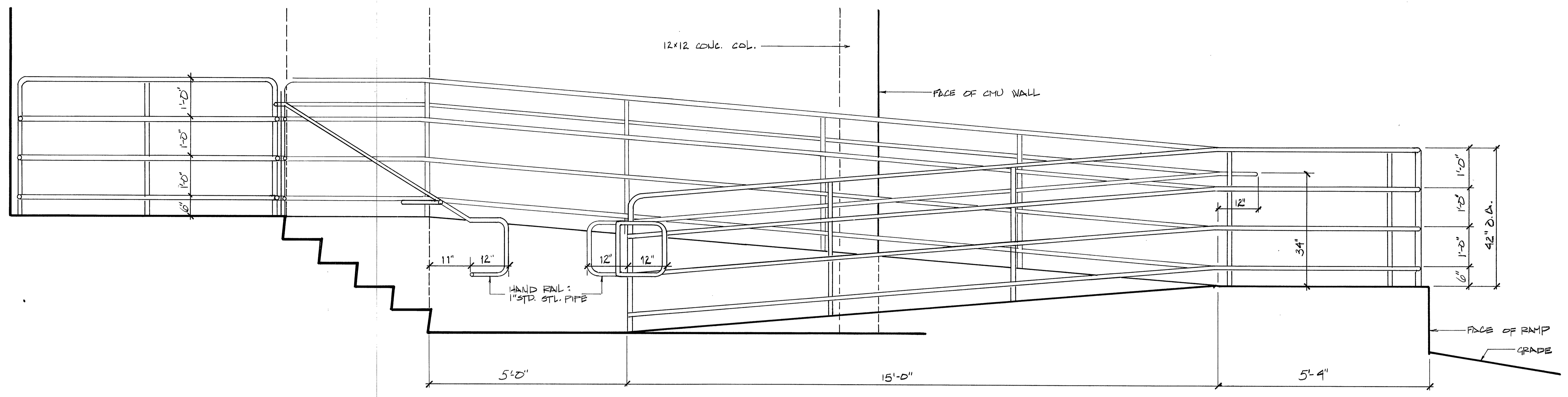
1 DETAIL-ELEVATION @ RAMP RAIL SCALE 3/4" = 1'-0"
