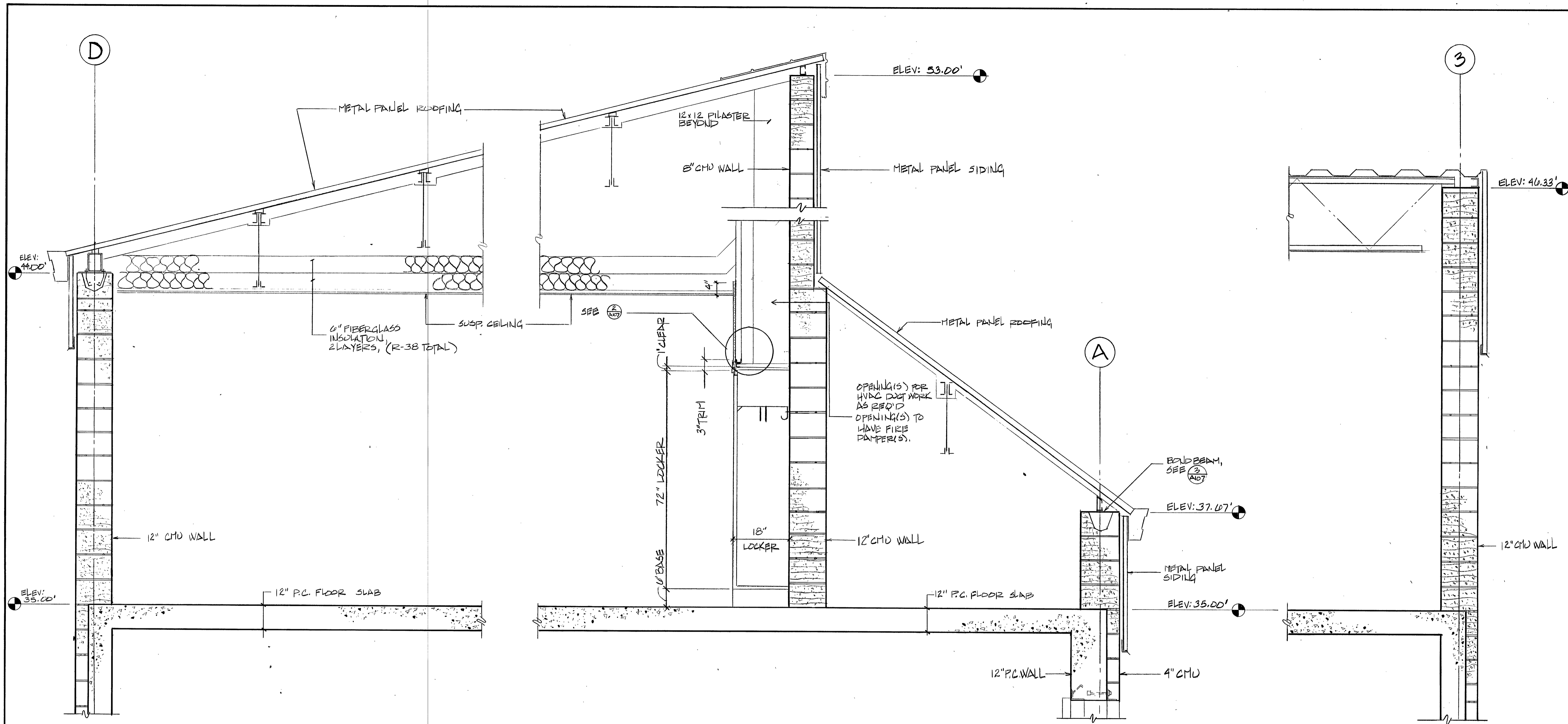
1 WEST WALL DETAIL A108 SCALE 3/4" = 1'-0"
