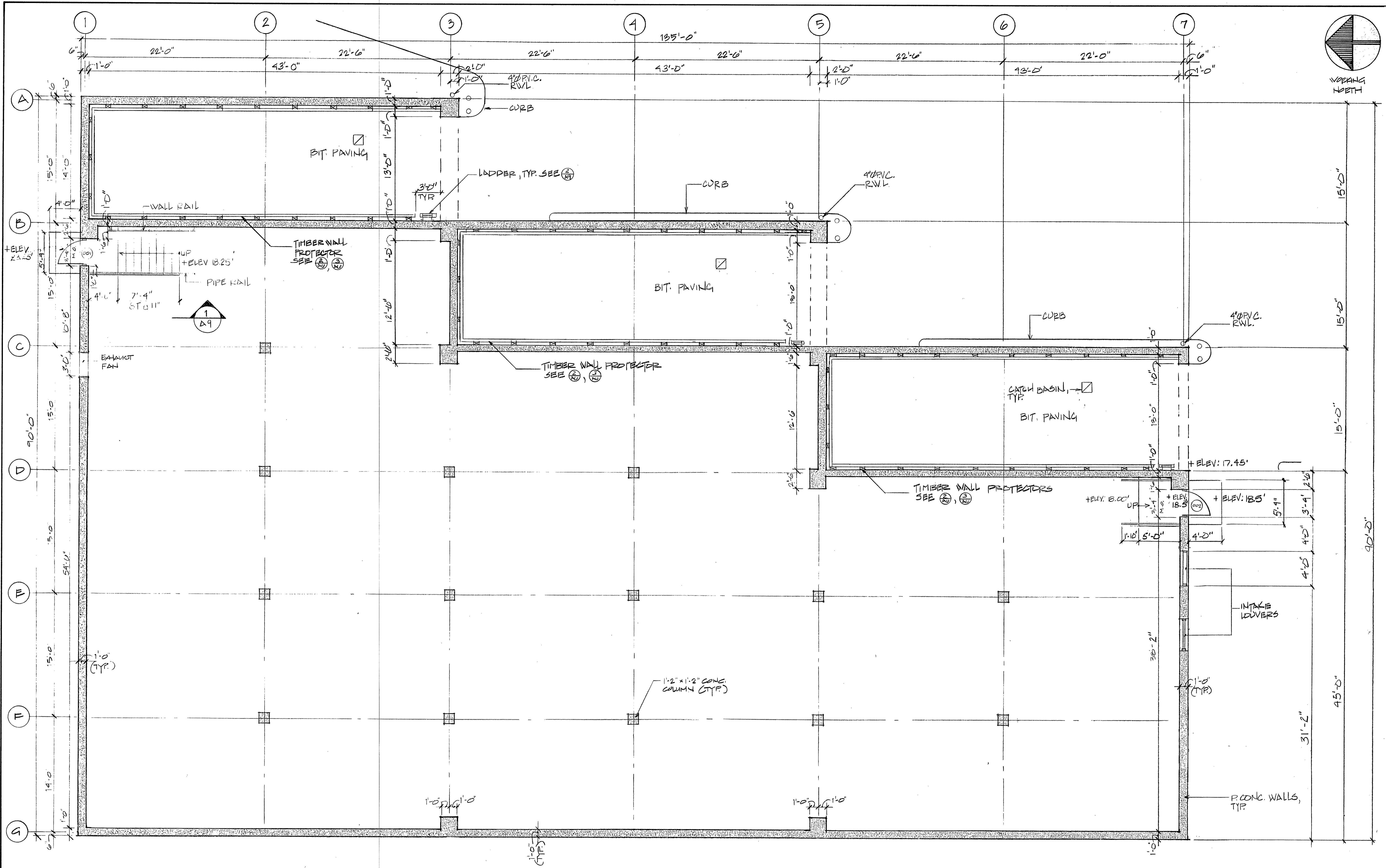
1 LOWER LEVEL FLOOR PLAN A1 SCALE 3/16" = 1'-0"
