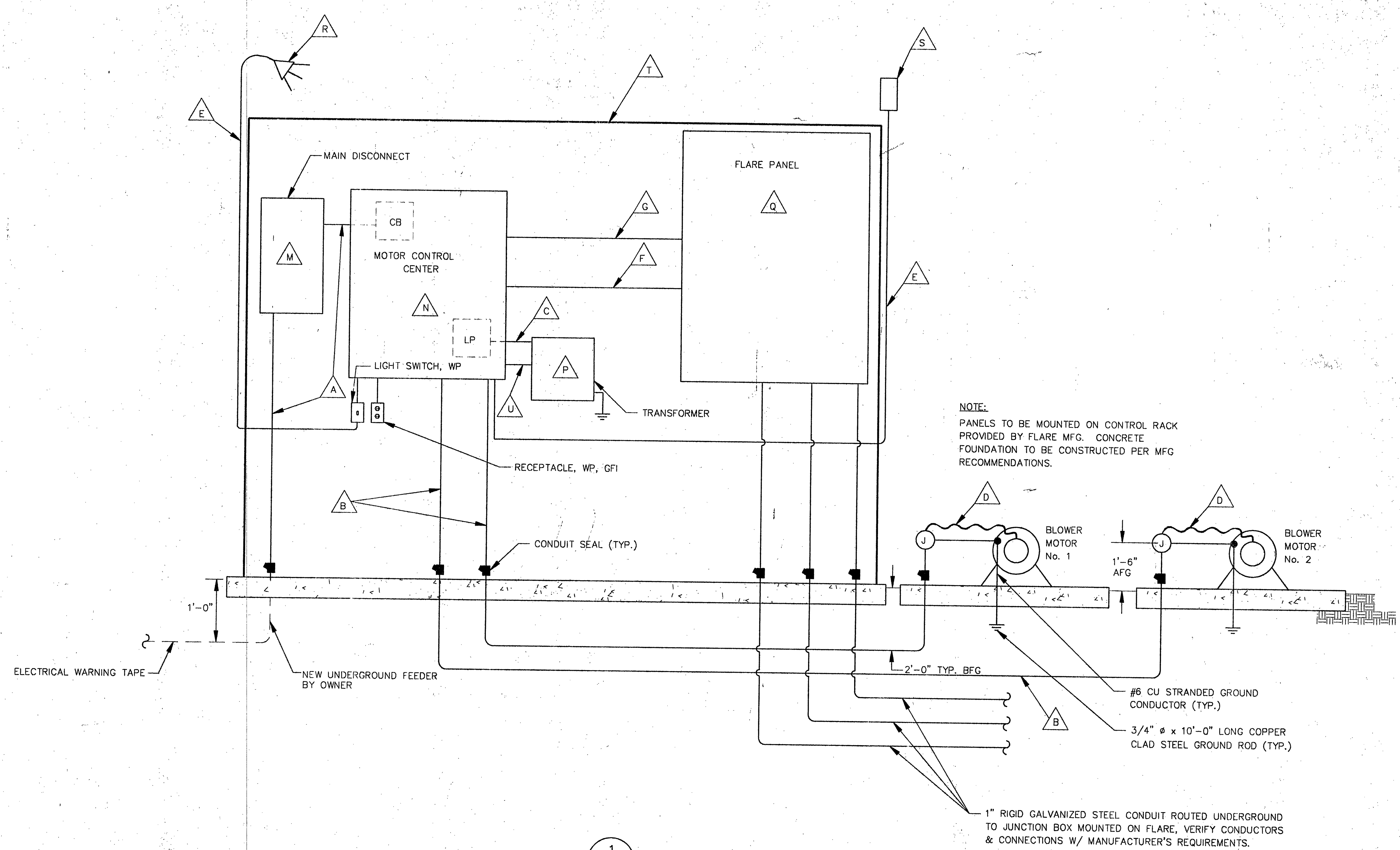
1 ELECTRICAL RISER DIAGRAM 15 NO SCALE
