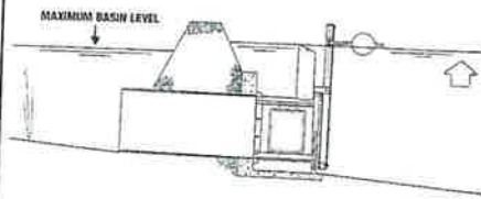
4. NORMAL HIGH TIDE GATE FULLY CLOSED
