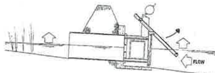
2. RISING TIDE FLOATS GATE UP FLOODING ESTUARY BASIN
