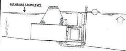
4. AT NORMAL TIDE LEVEL GATE IS CLOSED
