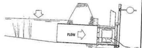
6. RECEDING TIDE - SIDE FLAPS OPEN TO ALLOW DRAINAGE OF ESTUARY - MAIN GATE COVER RESTRICTED TO PARTIALLY OPEN UNTIL NEXT TIDE
